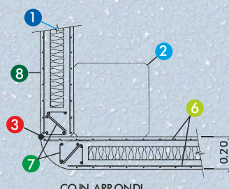
COIN ARRONDI
