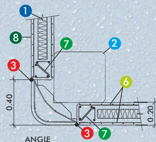
ANGLE
